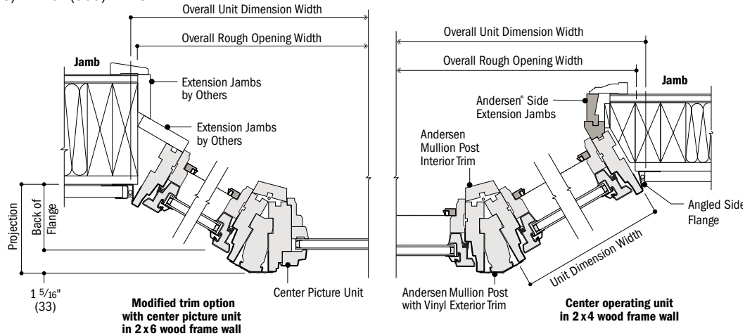
Horizontal Section
