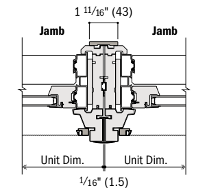
Horizontal Section Tilt-Wash Double-Hung to Tilt-Wash Double-Hung
