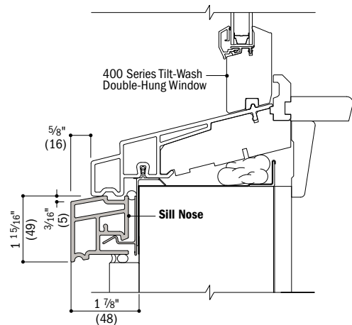
Vertical Section
