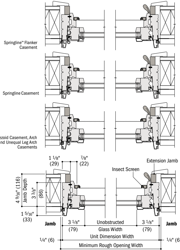
Horizontal Section Casement
