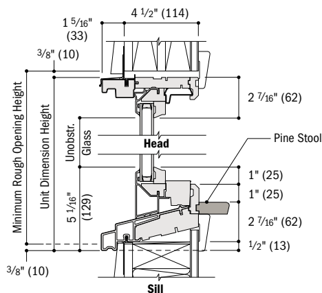
Vertical Section
