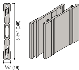
\frac{3}{4} " (19) x 5\frac{3}{4} " (146) Fiberglass Joining Material For 4\frac{9}{16} " (116) jamb depths.
