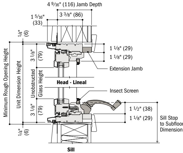
Vertical Section Casement
