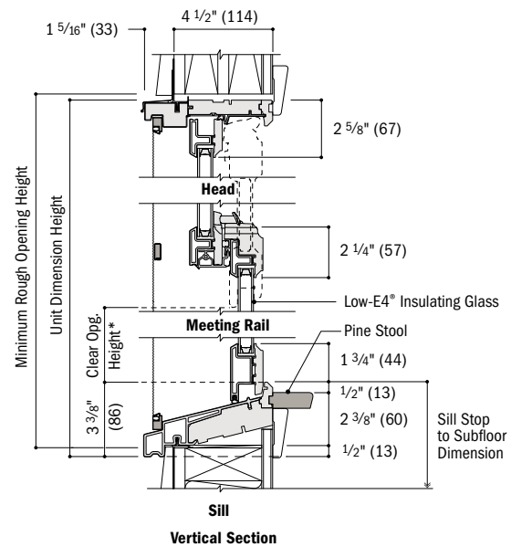
Vertical Section
