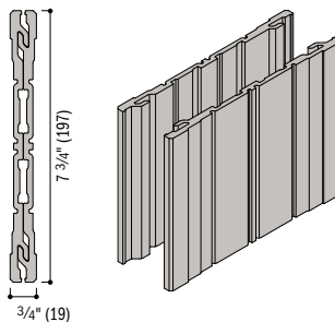
\frac{3}{4} " (19) x 7\frac{3}{4} " (197) Fiberglass Joining Material For higher performance for 1-way and 2-way joining. Required for Frenchwood® hinged inswing patio doors with 6\frac{9}{16} " (167) base jamb depths.
