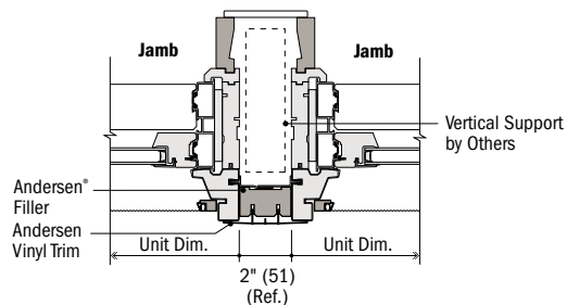
Horizontal Section Tilt-Wash Double-Hung and Tilt-Wash Double-Hung
